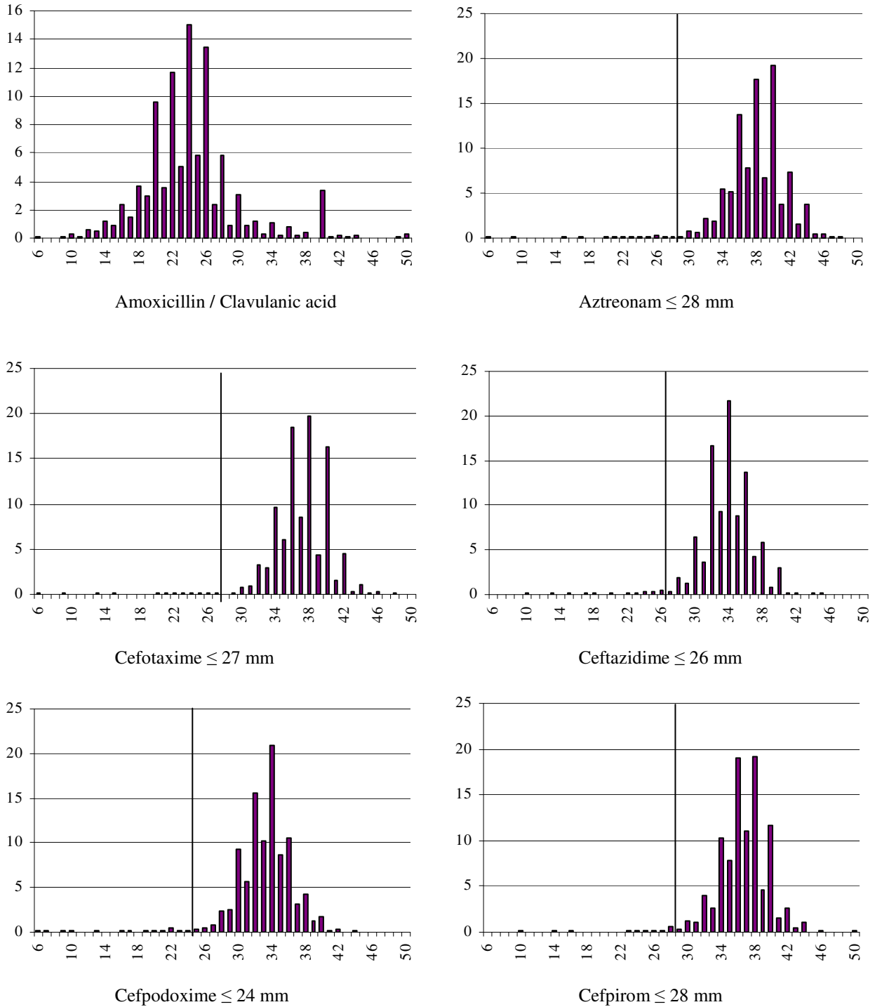
FIGURE 21. Distributions disk diffusion zone diameters (mm) of aztreonam, amoxicillin/clavulanic acid, cefotaxime, ceftazidime, cefpodoxime and cefpirom in E. coli from blood cultures and urine. Suggested cut-off values for ESBL detection are represented by vertical black bars.
