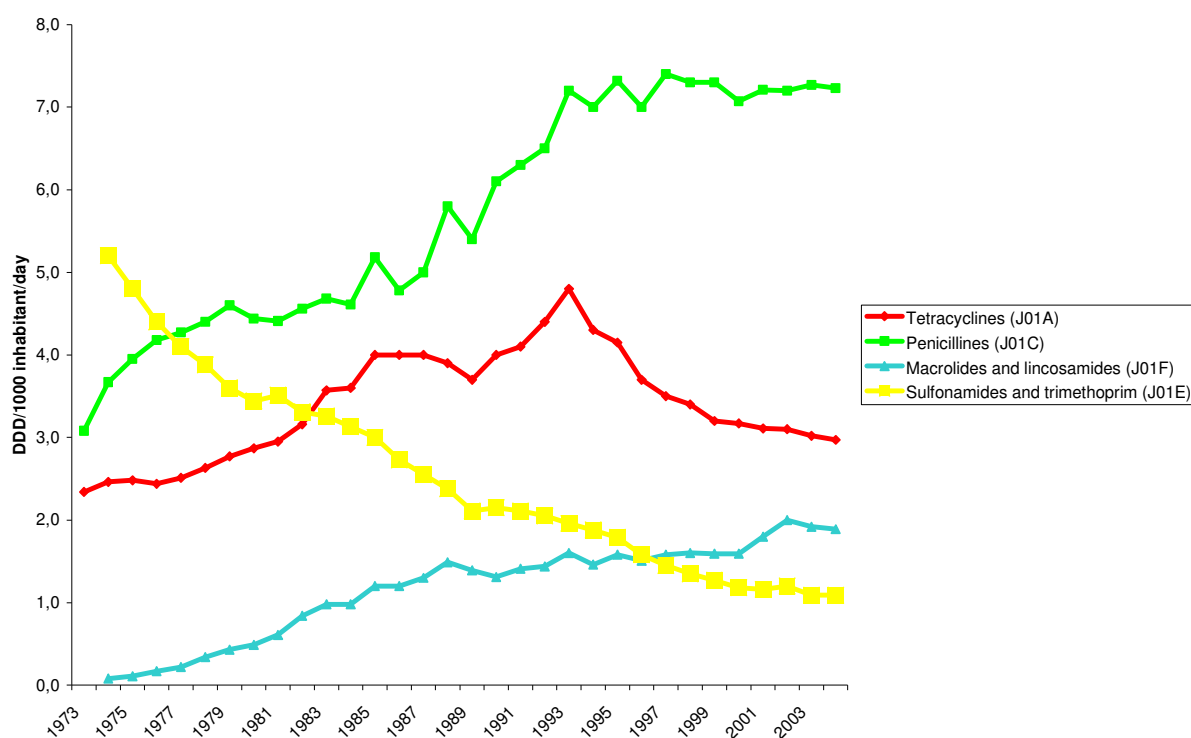
FIGURE 3. Sales of penicillins (J01C), tetracyclines (J01A), macrolides, lincosamides and streptogramins (J01F) and sulfonamides and trimethoprim (J01E) in Norway 1973-2004.
