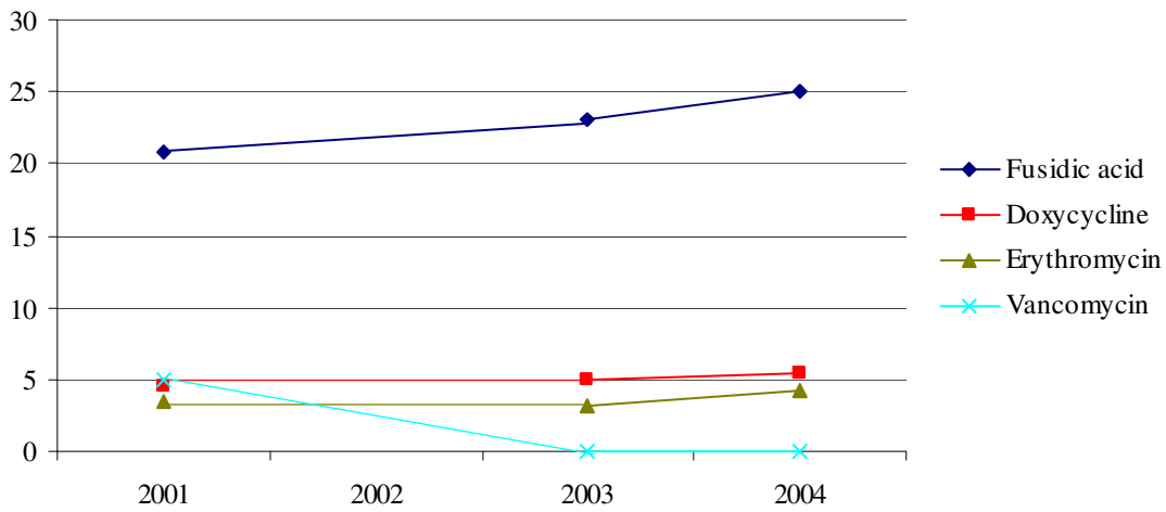
FIGURE 33. Prevalences (%) of non-susceptibility to various antibiotics other than beta-lactam in S. aureus isolates from wound specimens 2001 - 2004.
