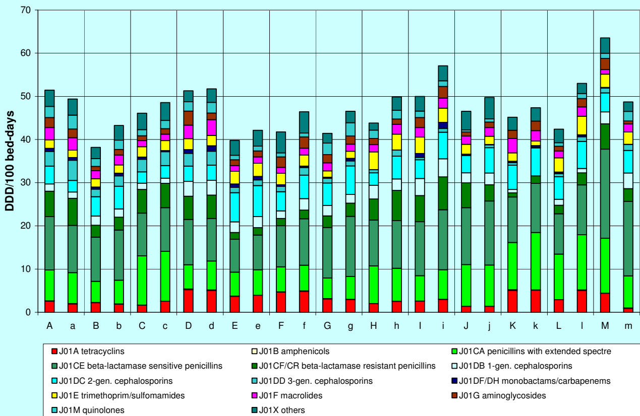
FIGURE 8. Usage of antibacterials in 13 Norwegian hospitals in 1998 (capital letters) and 1999 (small letters). Given in DDD/100 bed-days. ATC/DDD-version 2005 is used. Hospitals are ranged after size from large (A) to small (M).
